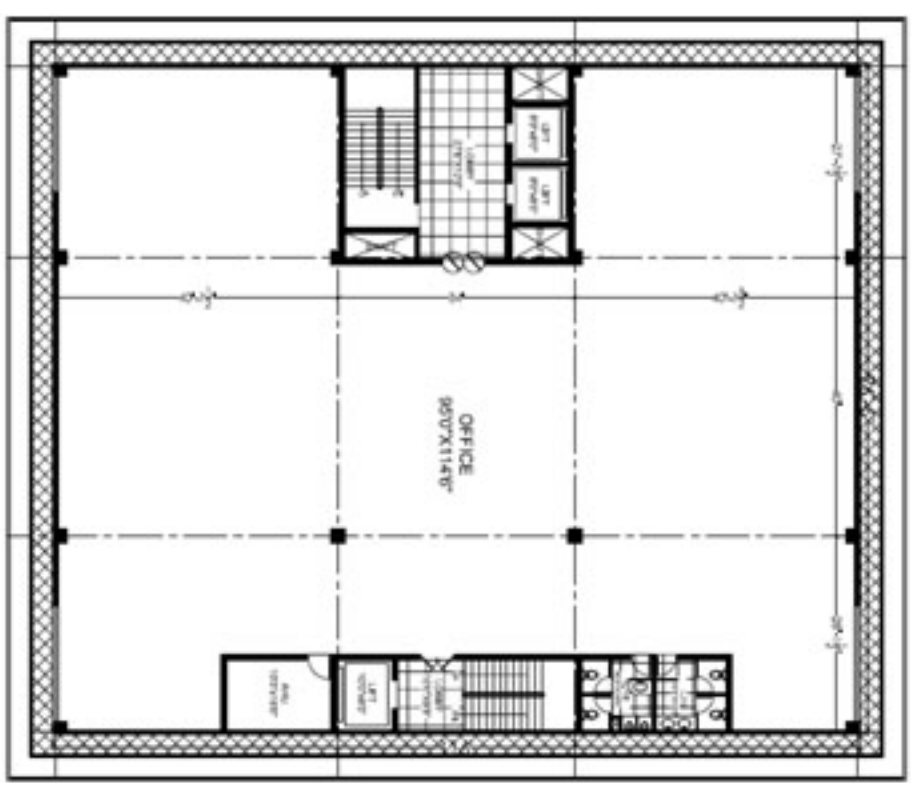
NINTH TO TWELFTH FLOOR PLAN (THIRD LVL.)
